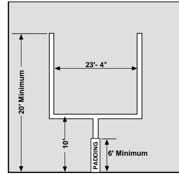
GOAL POST DETAIL
