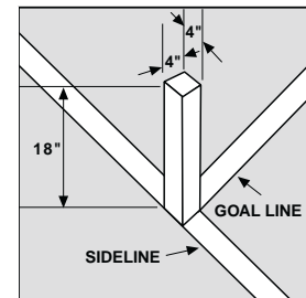
PYLON DETAIL
