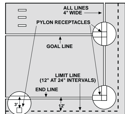
END ZONE DETAIL
